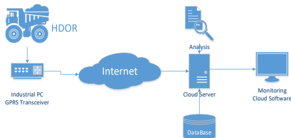
Figure 6: System schematic with GPRS Connection
